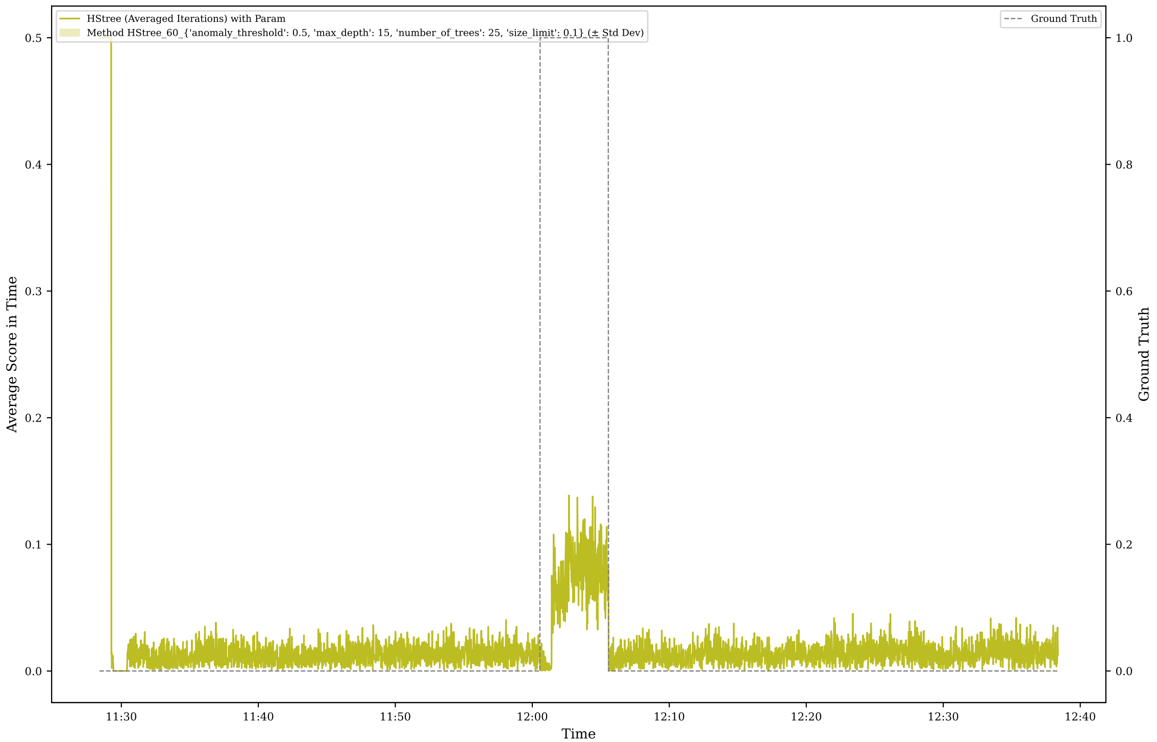
Method HStree Score for Scenario A8
